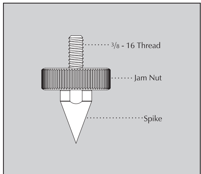
Figure 7. The ETC™ Spike.
